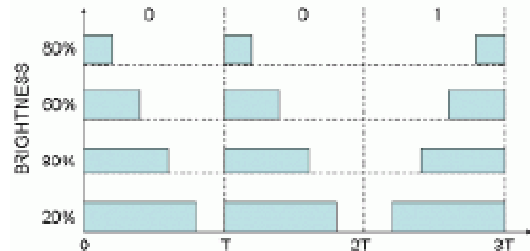
Variable Pulse Position Modulation (VPPM) supports dimming
